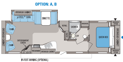
JAY FLIGHT G2 | 32RLS Ext. Length: 35' 5" Ext. Height: 134" Unloaded Weight (lbs.): 7,235
