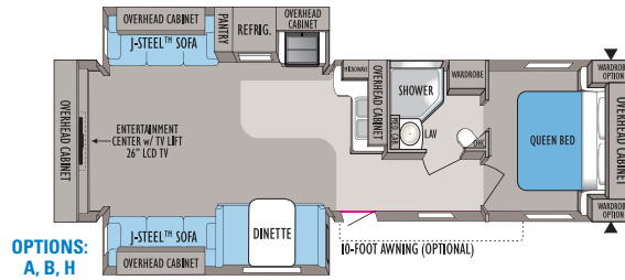
JAY FLIGHT G2 | 33RLDS Ext. Length: 35' 6" Ext. Height: 134" Unloaded Weight (lbs.): TBD
