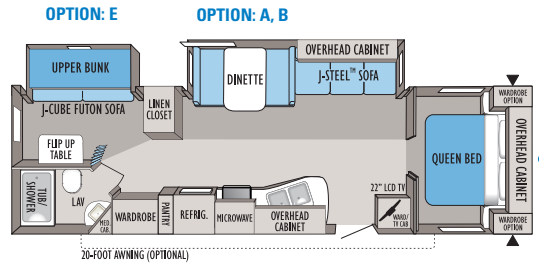
JAY FLIGHT G2 | 31BHDS Ext. Length: 33' 11" Ext. Height: 134" Unloaded Weight (lbs.): 7,340
