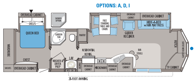
BUNGALOW | 40FER Ext. Length: 40' 11" Ext. Height: 152" Unloaded Weight (lbs.): 10,450
