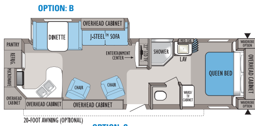
JAY FLIGHT G2 | 31RKS Ext. Length: 33' 8" Ext. Height: 134" Unloaded Weight (lbs.): 7,000
